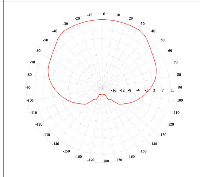
Azimuth @ 5.8GHz
