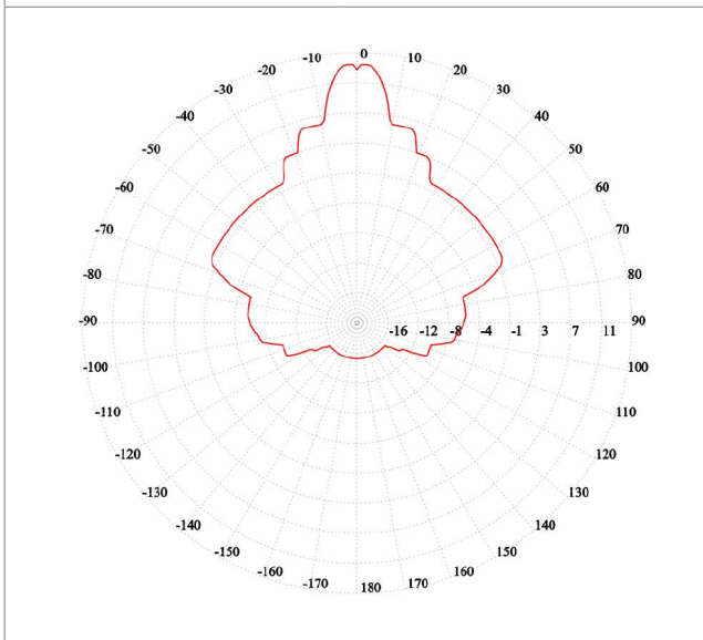
Elevation @ 5.8GHz
